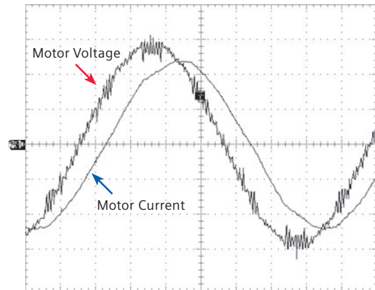
Multi-Level, Pulse-Width Modulated, Output-Voltage Waveform
