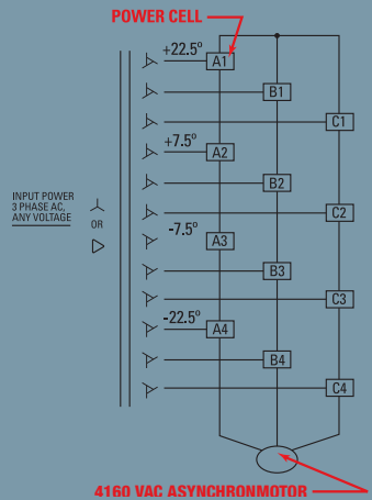
4160 VAC ASYNCHRONMOTOR
