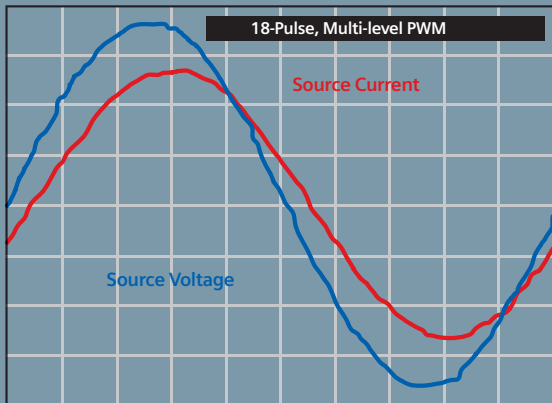
ROBICON Perfect Harmony Series Waveform
