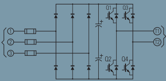
Power Cell
