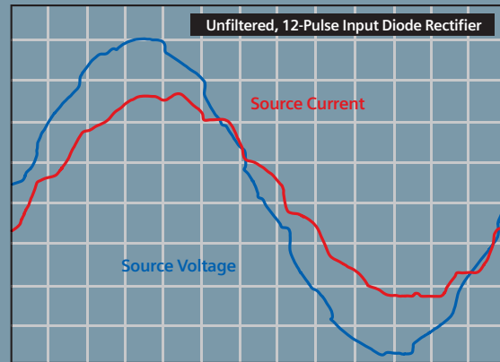
12-Pulse Harmonic Waveform
