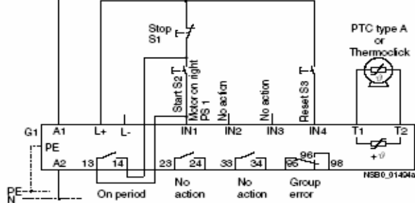
Control Circuit (Normal 1AC 230 V)
