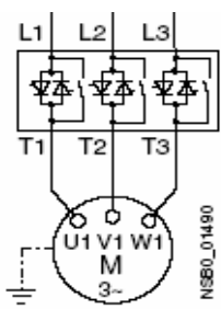
In-Line circuit
