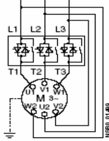
InSide Delta circuit
